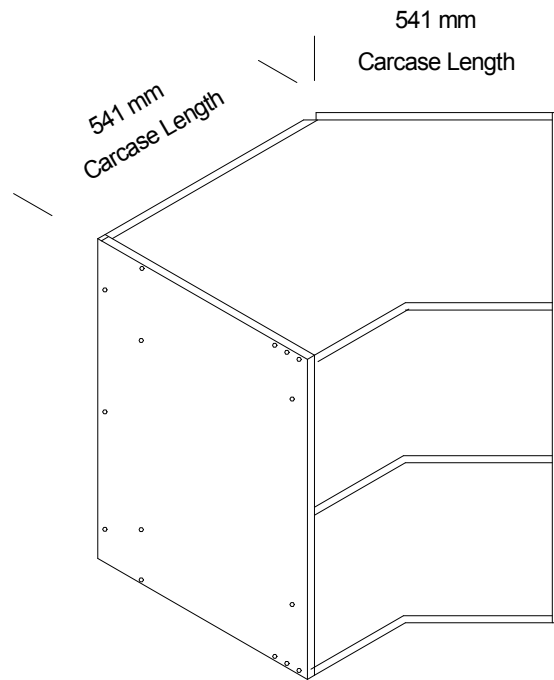
Isometric View
