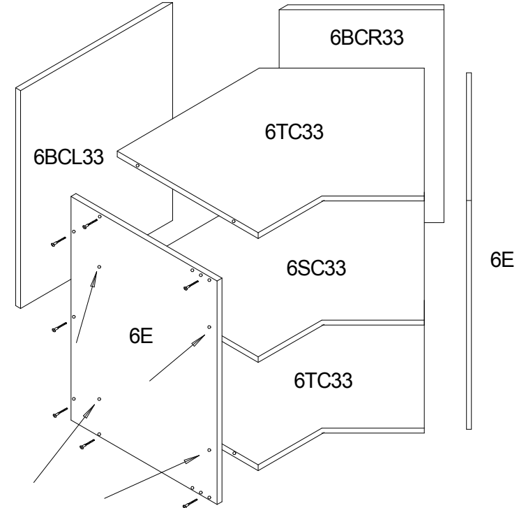
Exploded View
