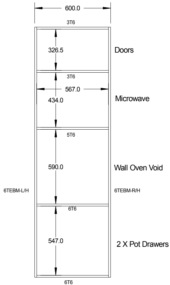
Front Elevation
